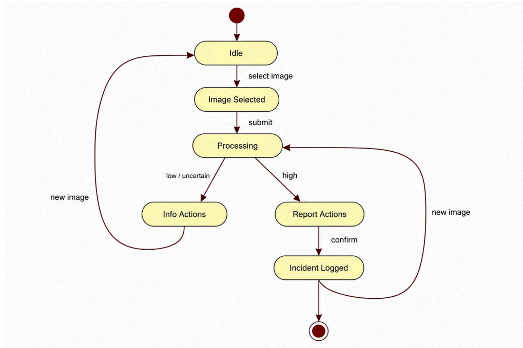
Figure 3.6: State transition diagram
