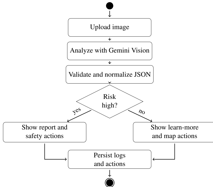
Figure 3.5: Activity diagram
