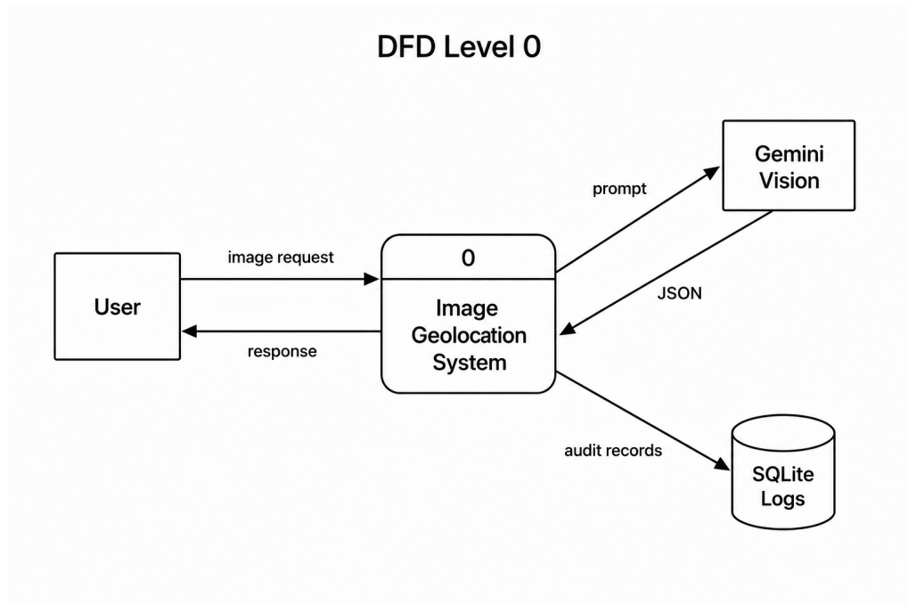
Figure 3.3: DFD Level 0 diagram
