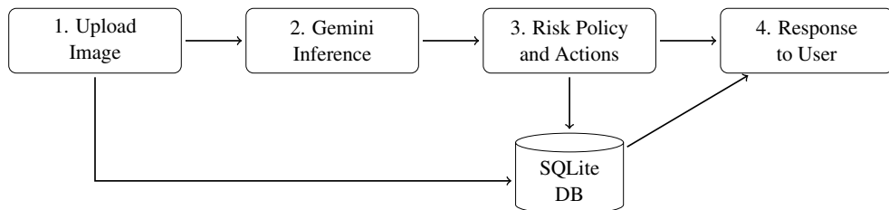
Figure 3.4: DFD Level 1 diagram
